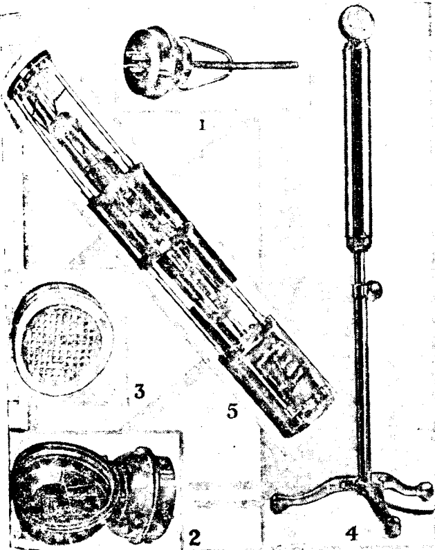
Left, components of the Remler microphone; and right, complete assembly.
