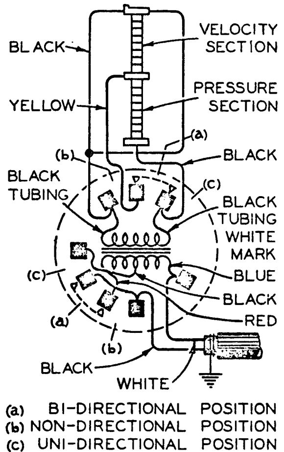
FIGURE 3 - MICROPHONE CIRCUIT (Schematic K-845900)
