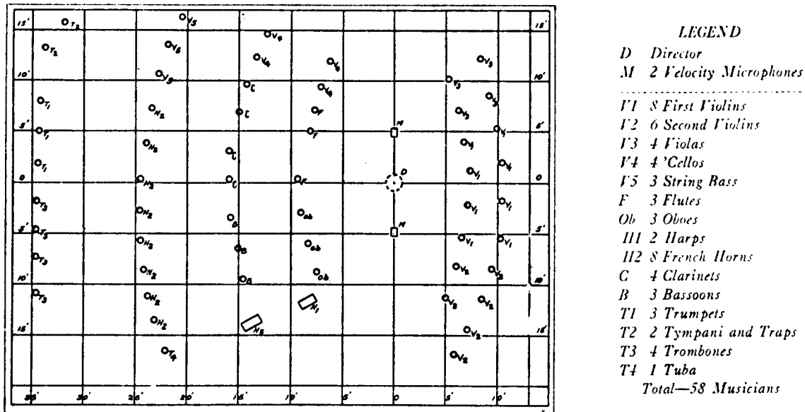
Figure 11—Microphone and Orchestra Arrangement for Symphony Orchestra
