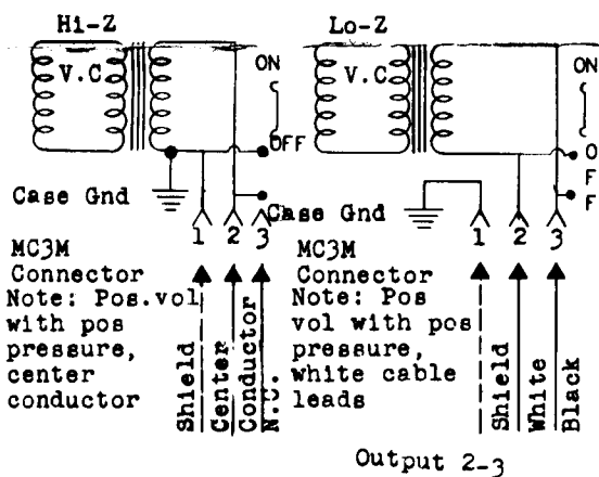
Fig. 5 — Wiring Diagram
