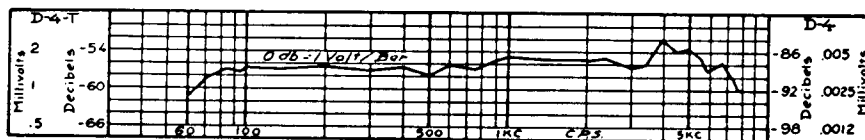
Average response of the D4 and D4T Dynamic Microphones for normal incident sound.
